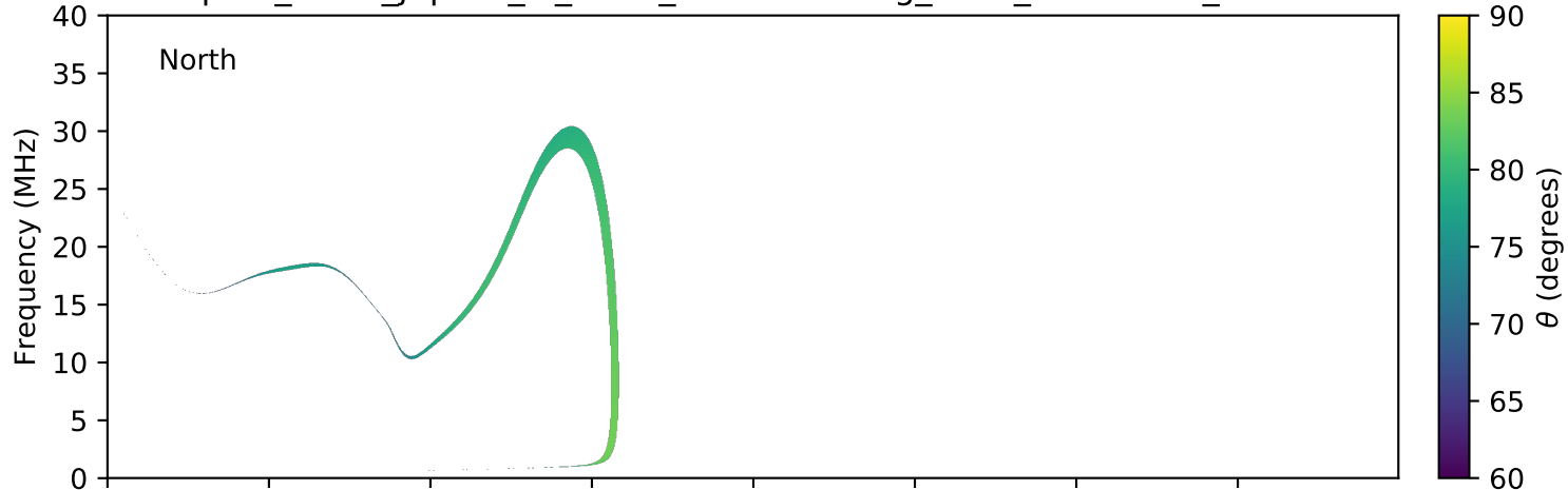
expres_earth_jupiter_io_isaac_lossc-wid1deg_3kev_20081225_v01.cdf
