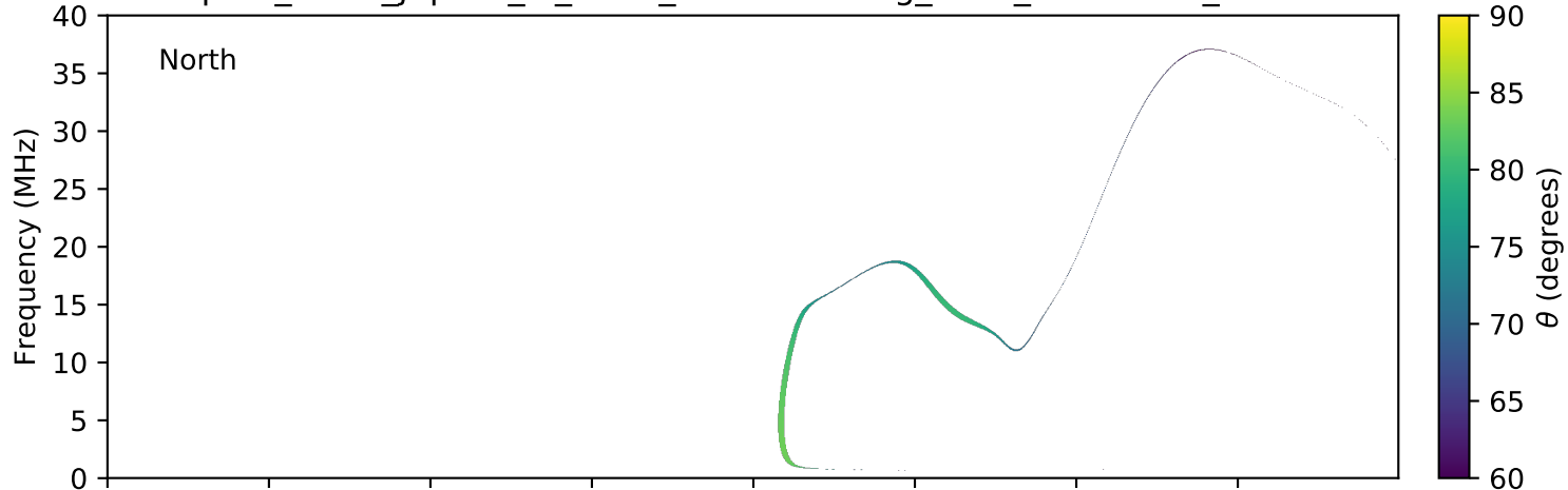
expres_earth_jupiter_io_isaac_lossc-wid1deg_3kev_20081224_v01.cdf
