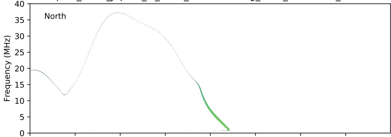
expres_earth_jupiter_io_isaac_lossc-wid1deg_3kev_20081223_v01.cdf
