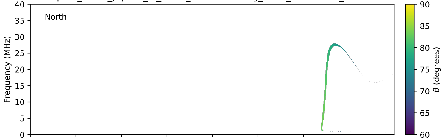
expres_earth_jupiter_io_isaac_lossc-wid1deg_3kev_20081222_v01.cdf
