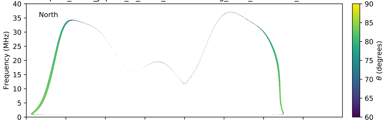
expres_earth_jupiter_io_isaac_lossc-wid1deg_3kev_20081221_v01.cdf
