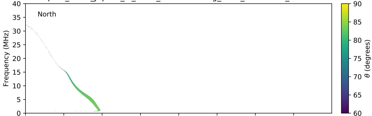
expres_earth_jupiter_io_isaac_lossc-wid1deg_3kev_20081218_v01.cdf
