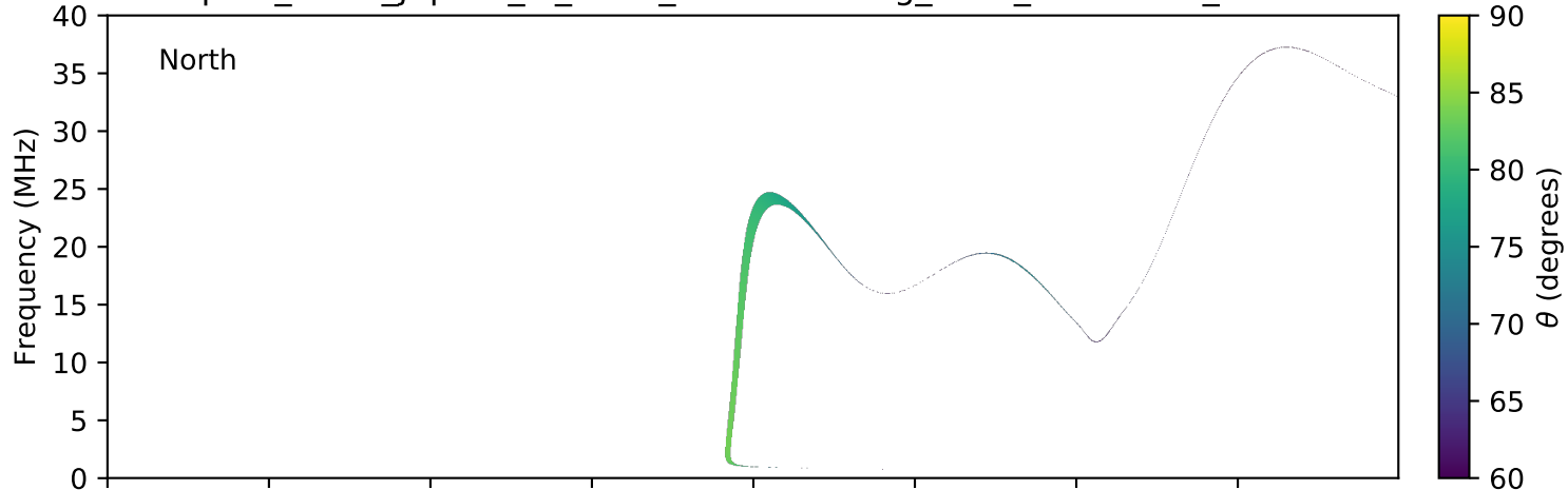
expres_earth_jupiter_io_isaac_lossc-wid1deg_3kev_20081217_v01.cdf
