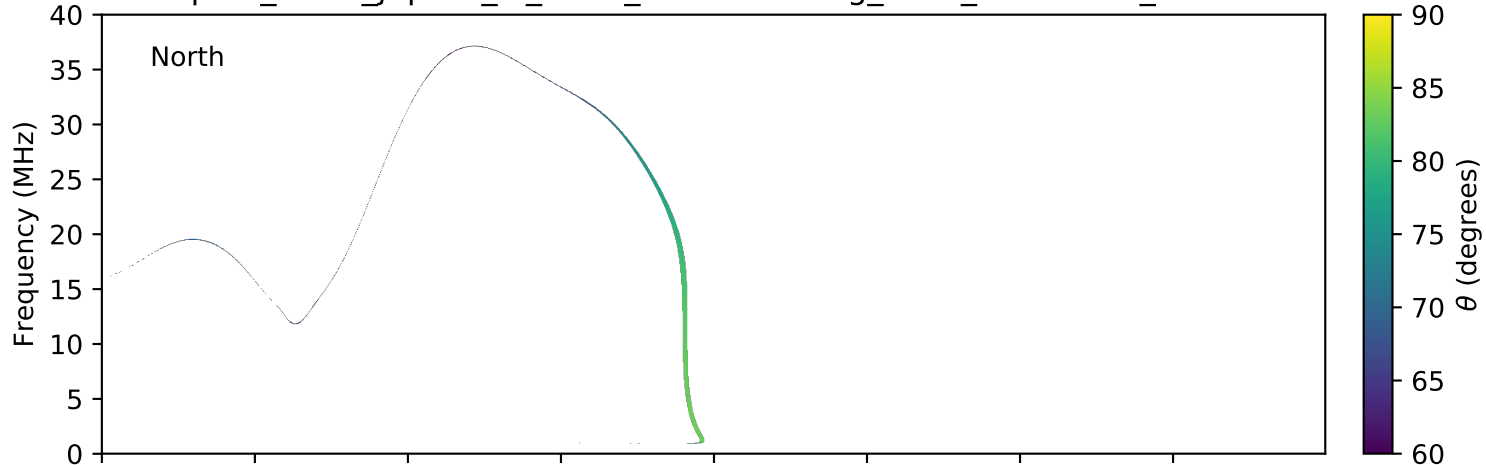
expres_earth_jupiter_io_isaac_lossc-wid1deg_3kev_20081216_v01.cdf
