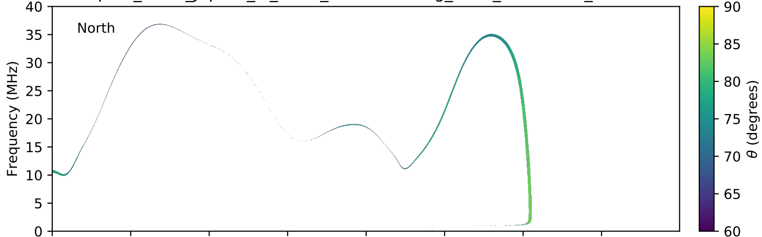
expres_earth_jupiter_io_isaac_lossc-wid1deg_3kev_20081214_v01.cdf
