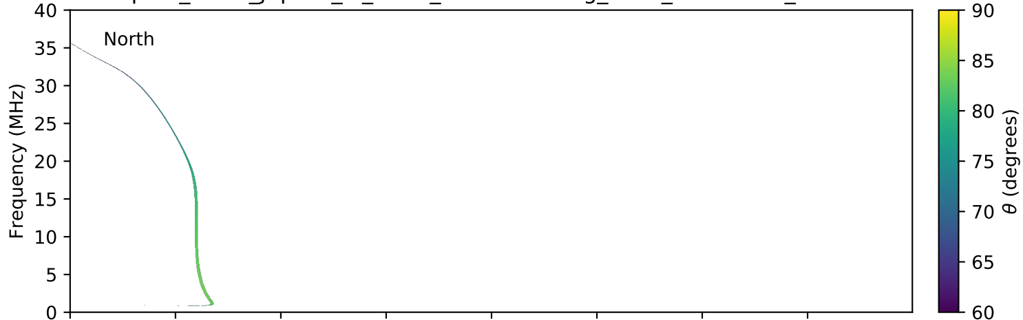
expres_earth_jupiter_io_isaac_lossc-wid1deg_3kev_20081211_v01.cdf
