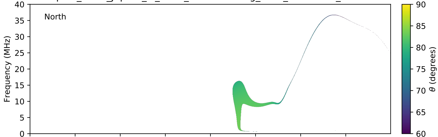
expres_earth_jupiter_io_isaac_lossc-wid1deg_3kev_20081208_v01.cdf
