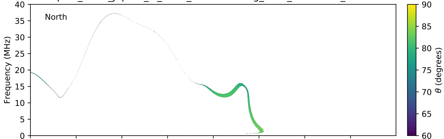
expres_earth_jupiter_io_isaac_lossc-wid1deg_3kev_20081207_v01.cdf
