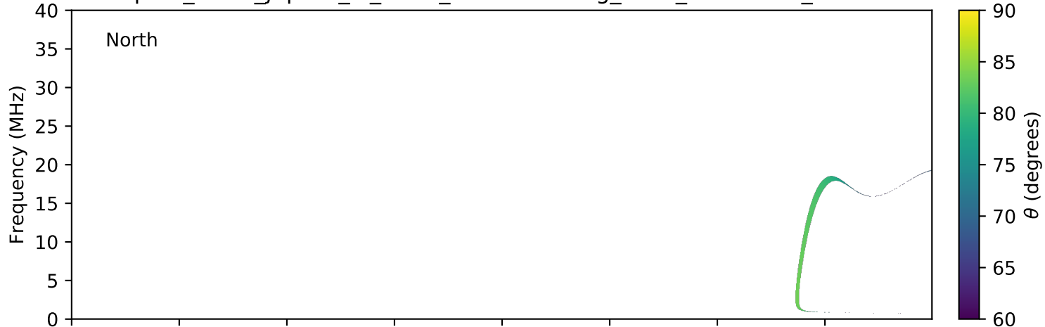
expres_earth_jupiter_io_isaac_lossc-wid1deg_3kev_20081206_v01.cdf
