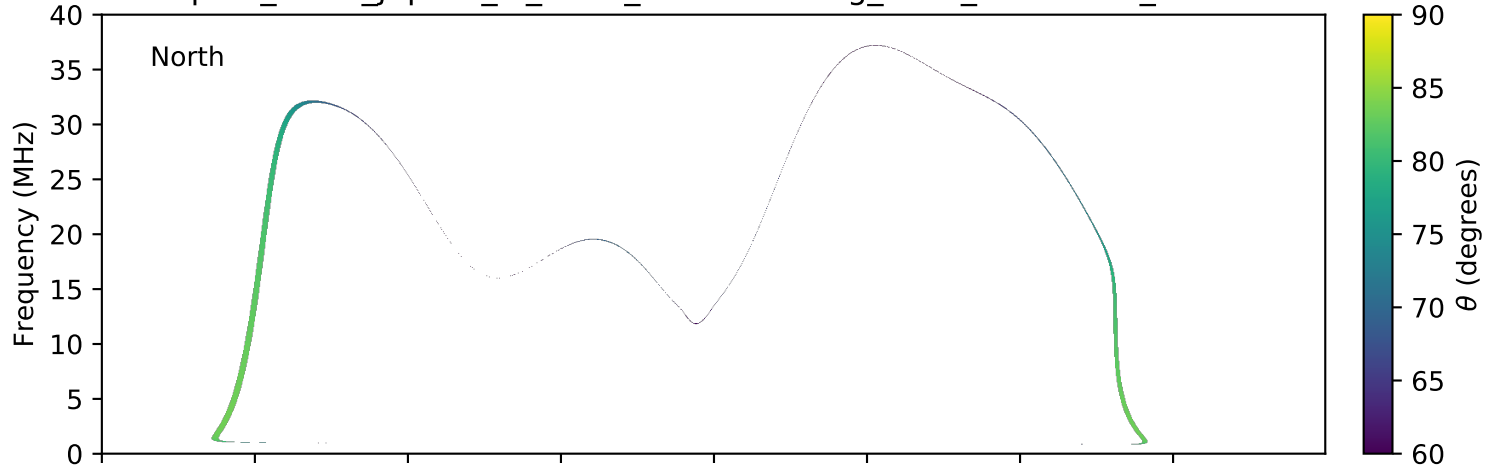
expres_earth_jupiter_io_isaac_lossc-wid1deg_3kev_20081205_v01.cdf
