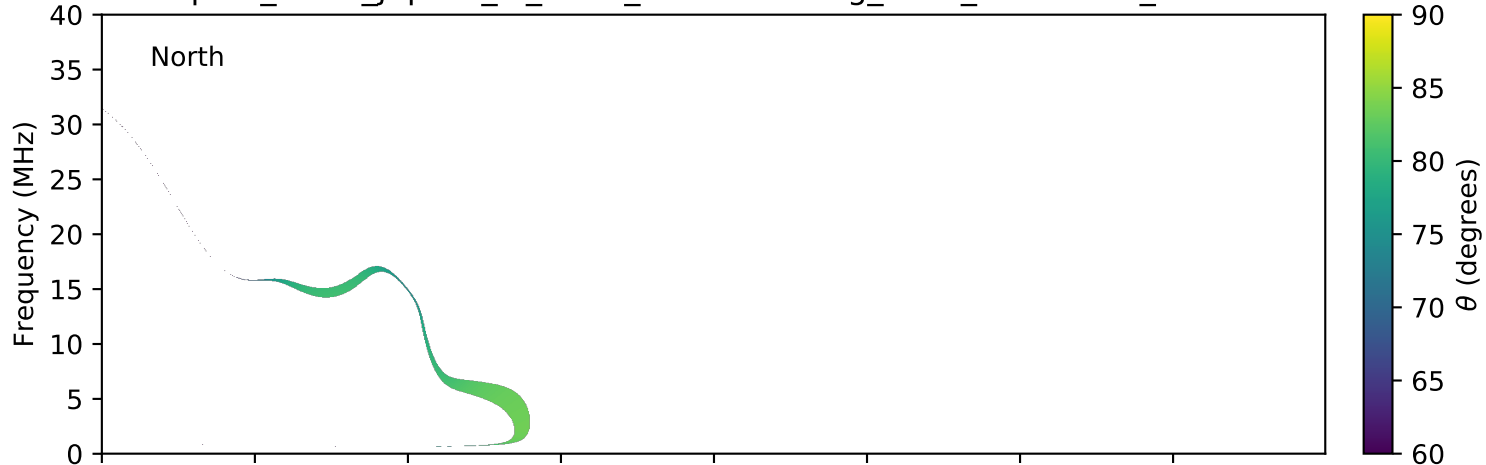
expres_earth_jupiter_io_isaac_lossc-wid1deg_3kev_20081202_v01.cdf
