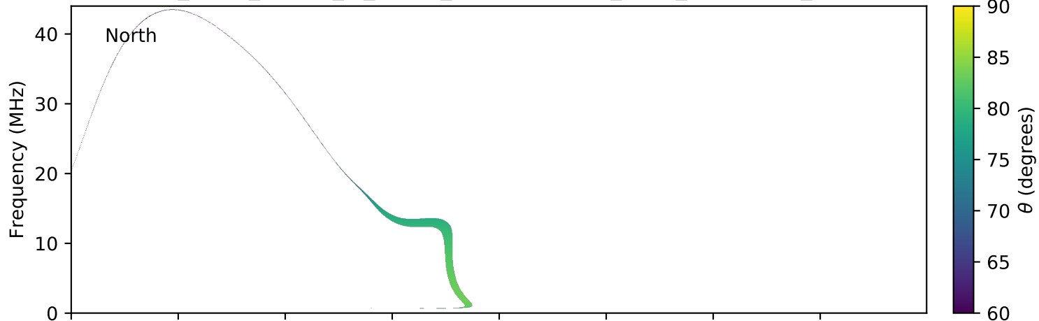
expres_earth_jupiter_io_jrm09_lossc-wid1deg_3kev_20081031_v01.cdf
