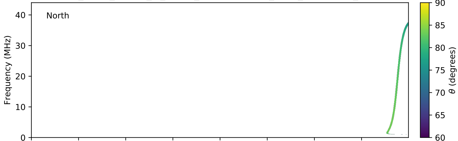
expres_earth_jupiter_io_jrm09_lossc-wid1deg_3kev_20081028_v01.cdf
