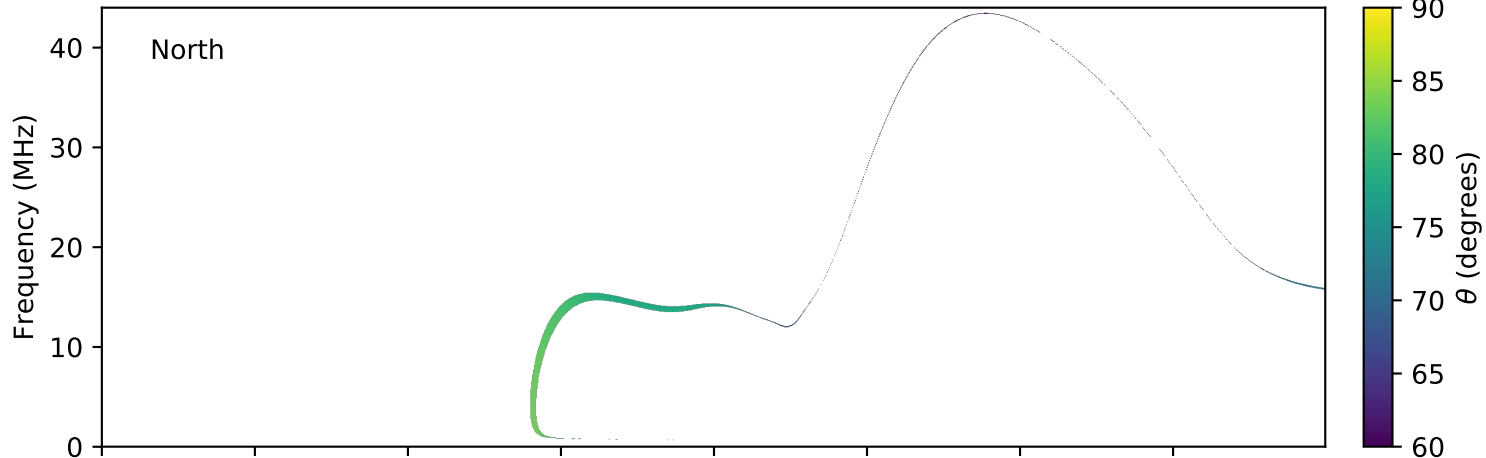
expres_earth_jupiter_io_jrm09_lossc-wid1deg_3kev_20081025_v01.cdf
