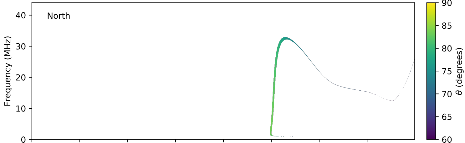
expres_earth_jupiter_io_jrm09_lossc-wid1deg_3kev_20081023_v01.cdf
