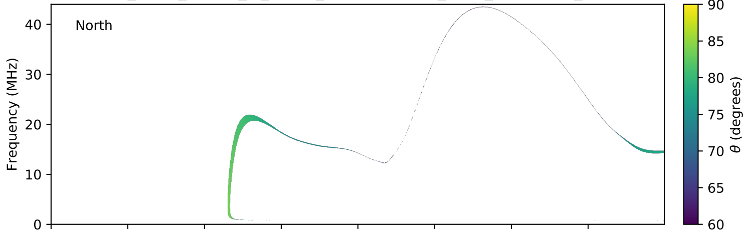
expres_earth_jupiter_io_jrm09_lossc-wid1deg_3kev_20081018_v01.cdf
