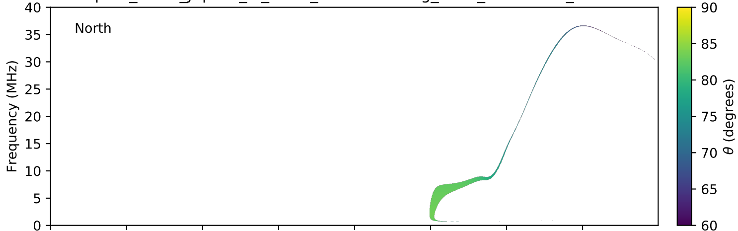
expres_earth_jupiter_io_isaac_lossc-wid1deg_3kev_20081030_v01.cdf
