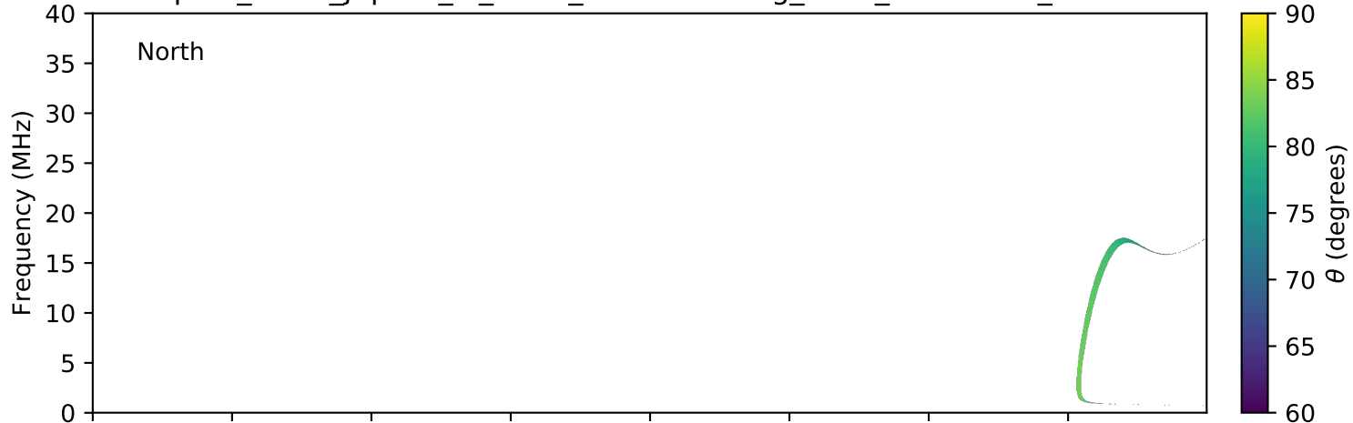
expres_earth_jupiter_io_isaac_lossc-wid1deg_3kev_20081028_v01.cdf
