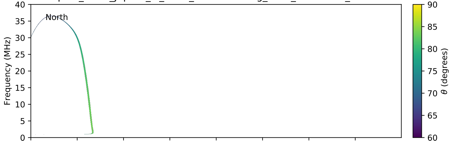
expres_earth_jupiter_io_isaac_lossc-wid1deg_3kev_20081026_v01.cdf
