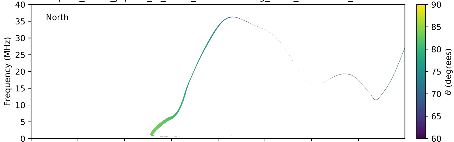
expres_earth_jupiter_io_isaac_lossc-wid1deg_3kev_20081025_v01.cdf
