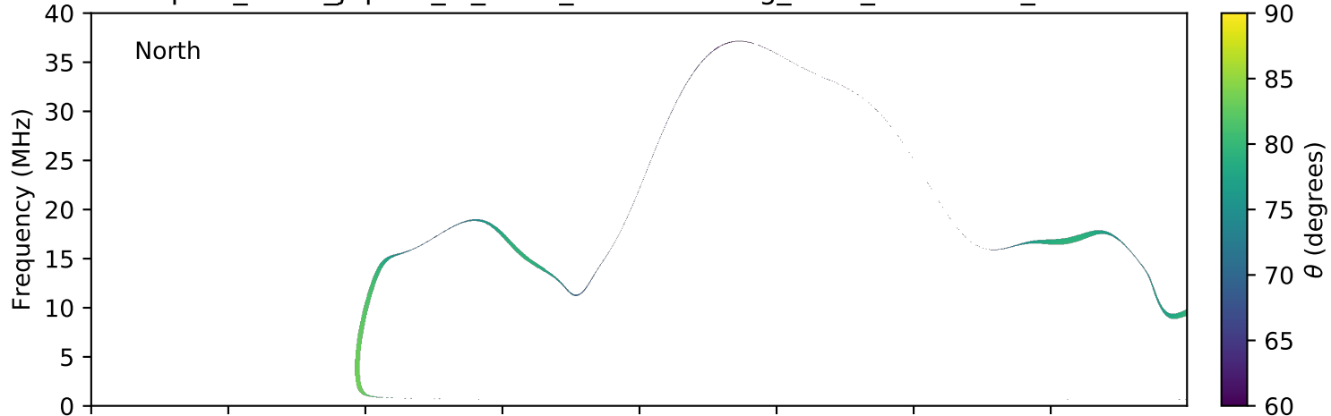
expres_earth_jupiter_io_isaac_lossc-wid1deg_3kev_20081018_v01.cdf
