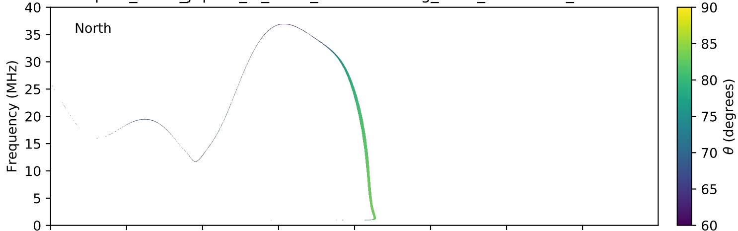
expres_earth_jupiter_io_isaac_lossc-wid1deg_3kev_20081015_v01.cdf
