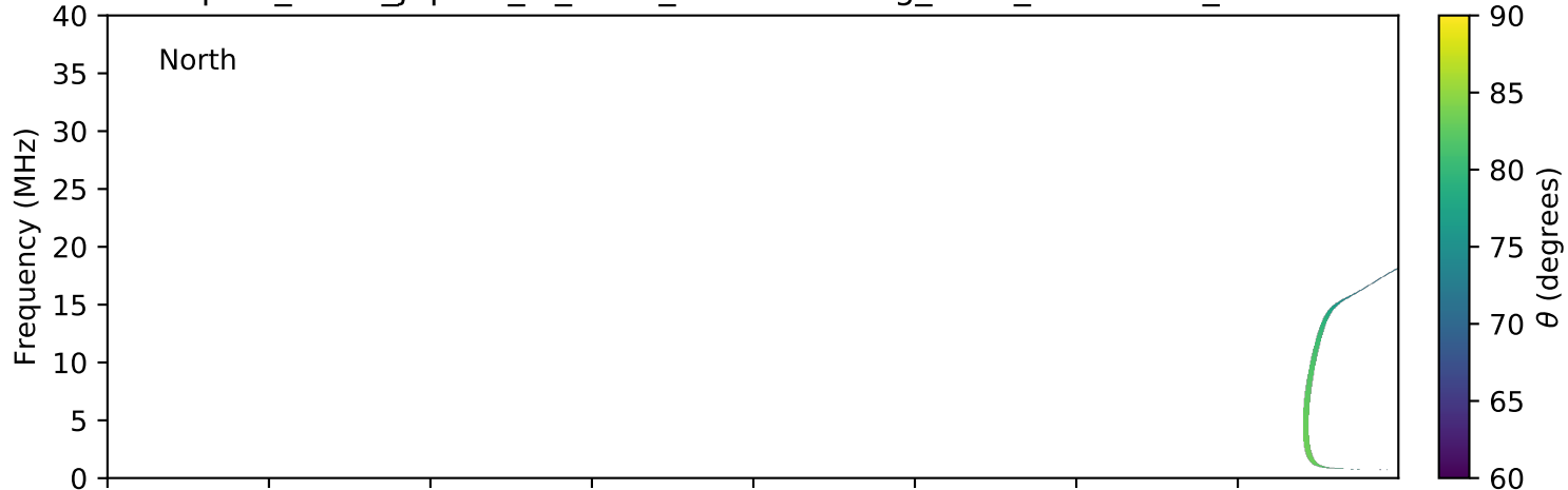
expres_earth_jupiter_io_isaac_lossc-wid1deg_3kev_20081012_v01.cdf
