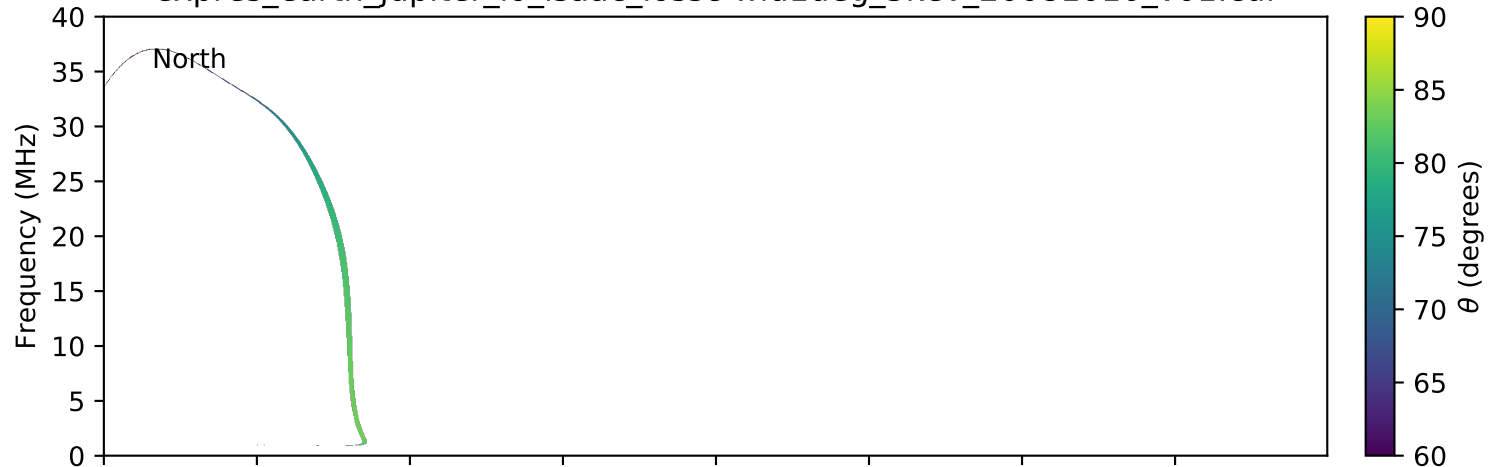
expres_earth_jupiter_io_isaac_lossc-wid1deg_3kev_20081010_v01.cdf
