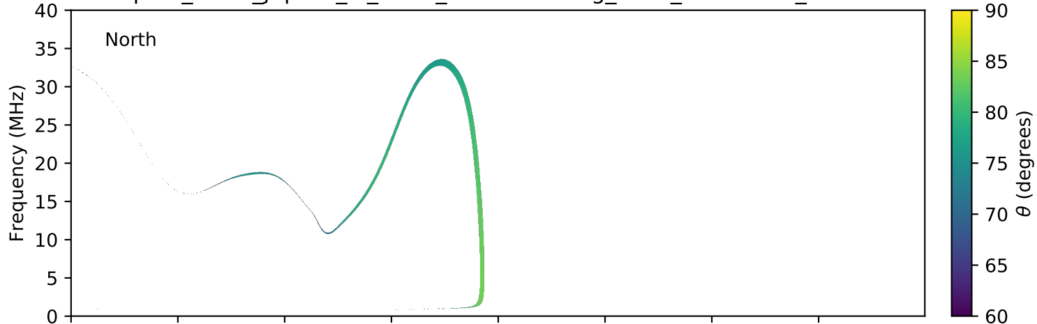
expres_earth_jupiter_io_isaac_lossc-wid1deg_3kev_20081008_v01.cdf
