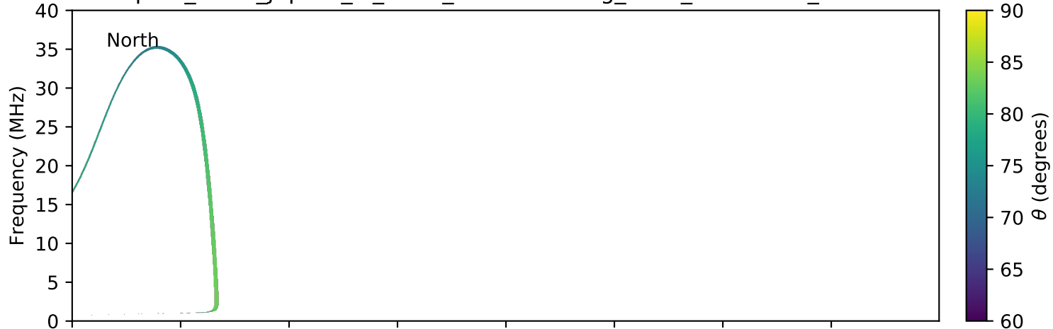
expres_earth_jupiter_io_isaac_lossc-wid1deg_3kev_20081003_v01.cdf
