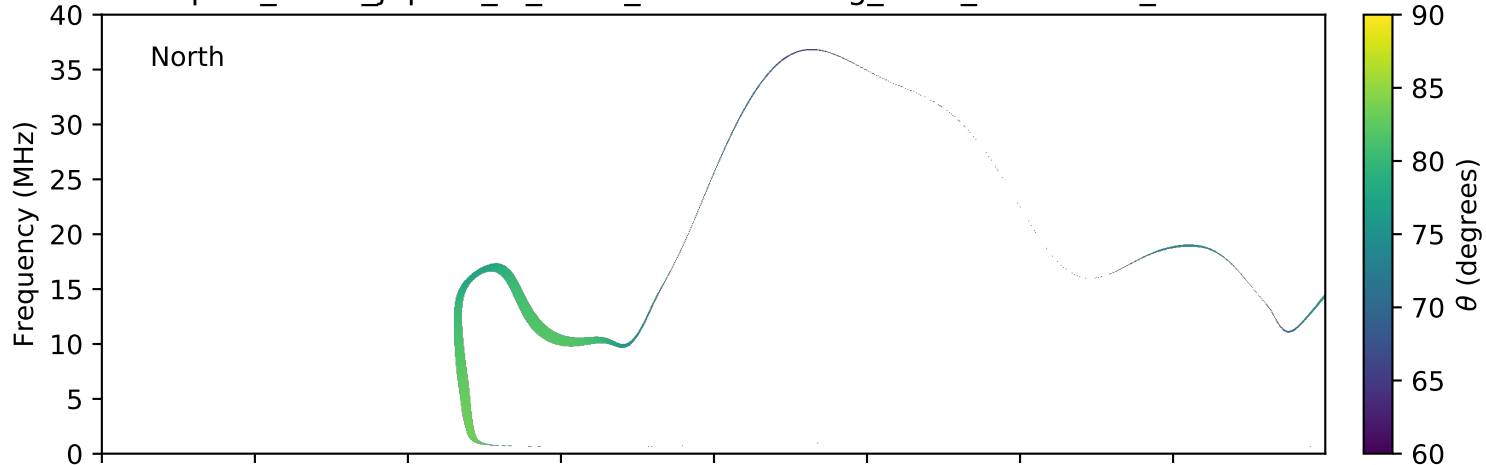
expres_earth_jupiter_io_isaac_lossc-wid1deg_3kev_20081002_v01.cdf
