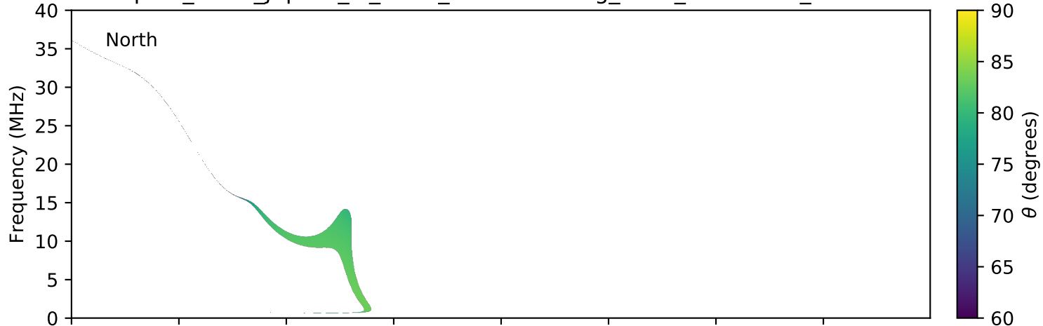
expres_earth_jupiter_io_isaac_lossc-wid1deg_3kev_20081001_v01.cdf
