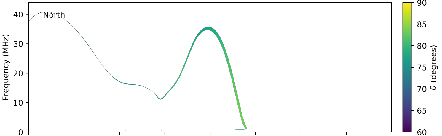
expres_earth_jupiter_europa_jrm09_lossc-wid1deg_3kev_20081022_v01.cdf
