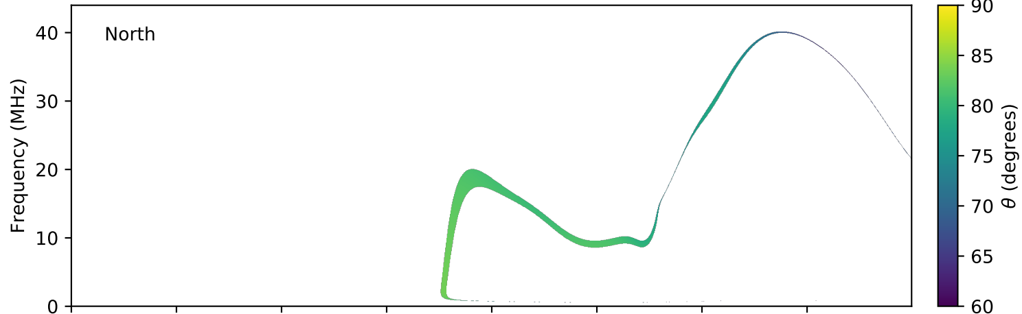
expres_earth_jupiter_europa_jrm09_lossc-wid1deg_3kev_20081017_v01.cdf
