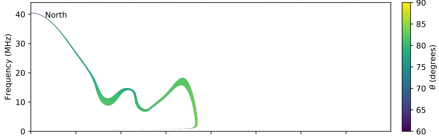
expres_earth_jupiter_europa_jrm09_lossc-wid1deg_3kev_20081008_v01.cdf
