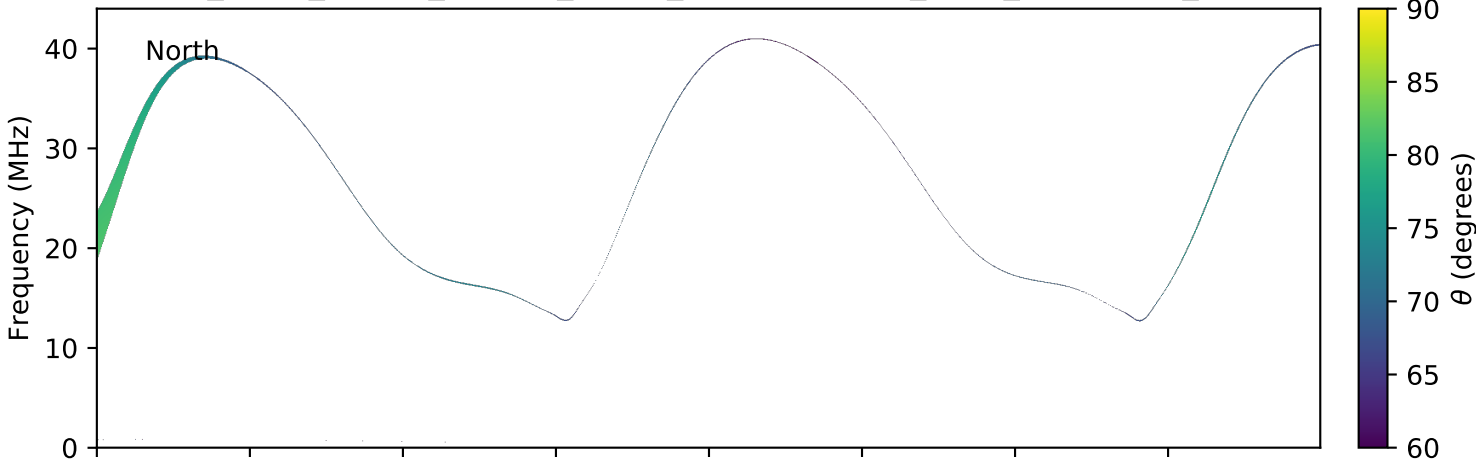
expres_earth_jupiter_europa_jrm09_lossc-wid1deg_3kev_20081007_v01.cdf
