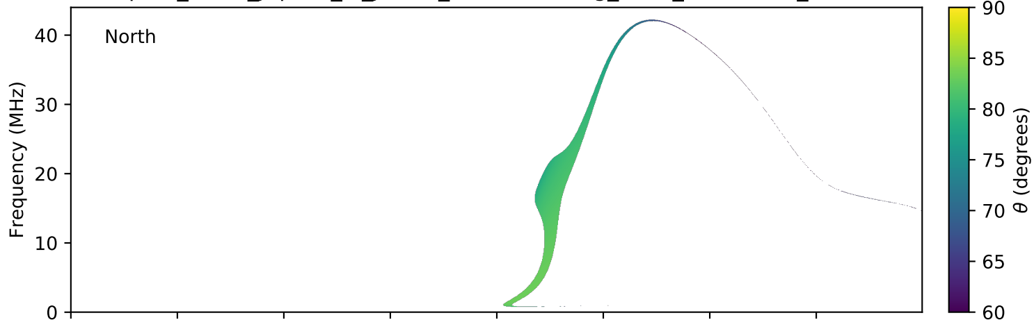
expres_earth_jupiter_io_jrm09_lossc-wid1deg_3kev_20080831_v01.cdf
