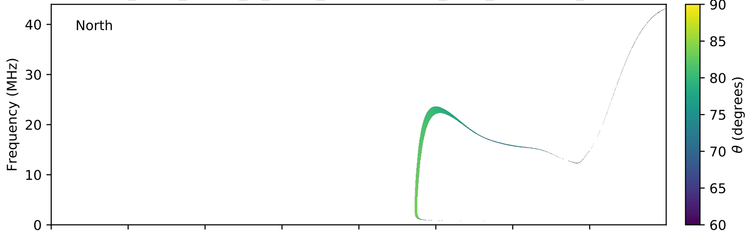
expres_earth_jupiter_io_jrm09_lossc-wid1deg_3kev_20080815_v01.cdf
