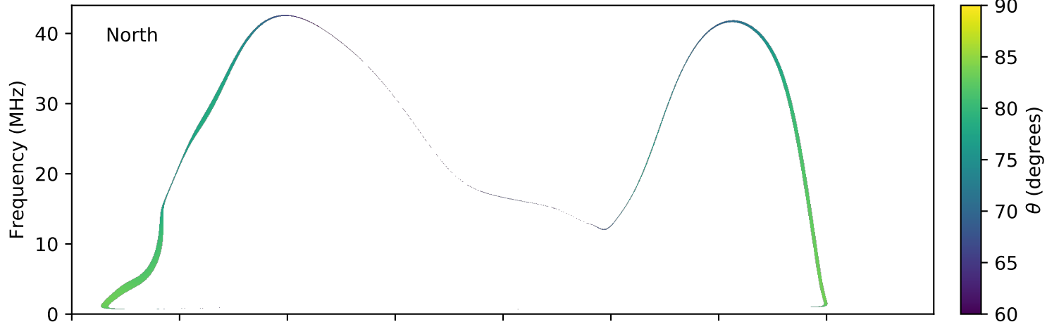
expres_earth_jupiter_io_jrm09_lossc-wid1deg_3kev_20080812_v01.cdf
