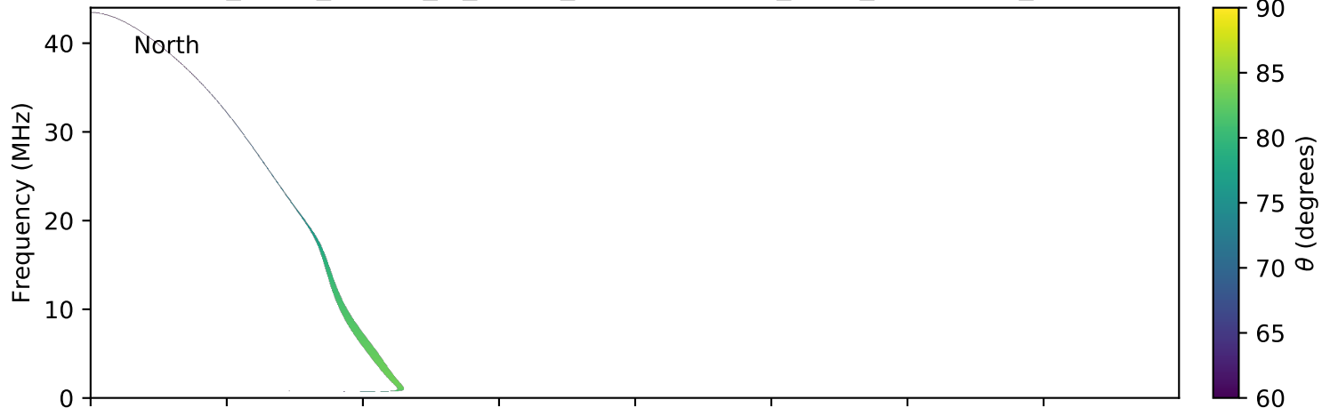
expres_earth_jupiter_io_jrm09_lossc-wid1deg_3kev_20080809_v01.cdf
