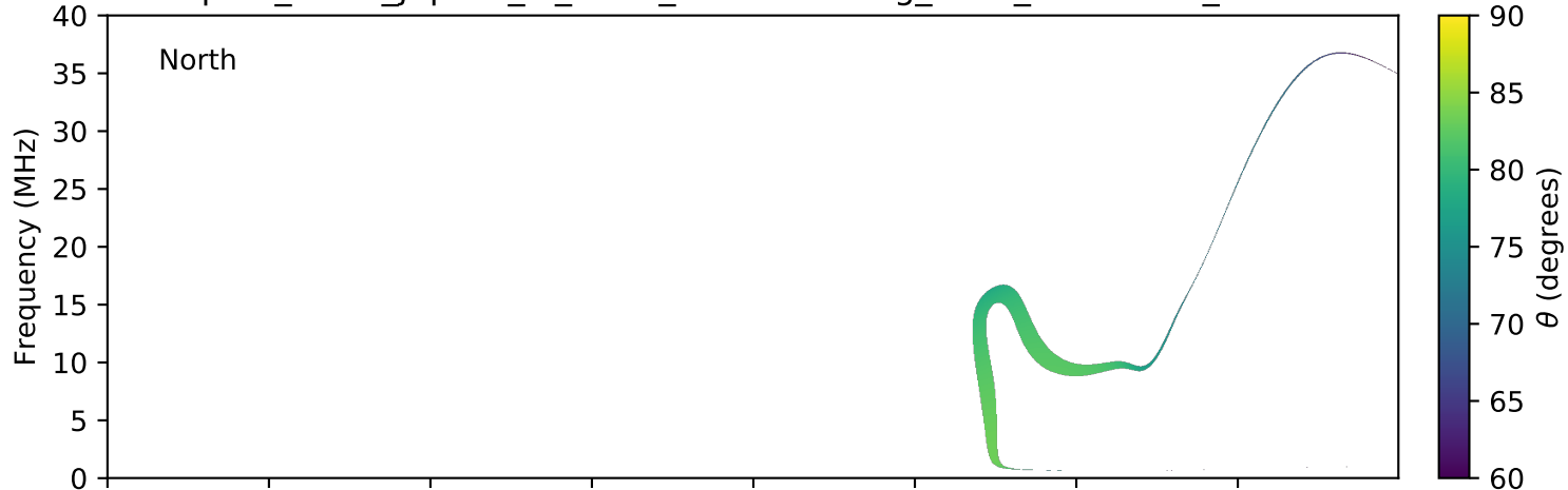
expres_earth_jupiter_io_isaac_lossc-wid1deg_3kev_20080829_v01.cdf
