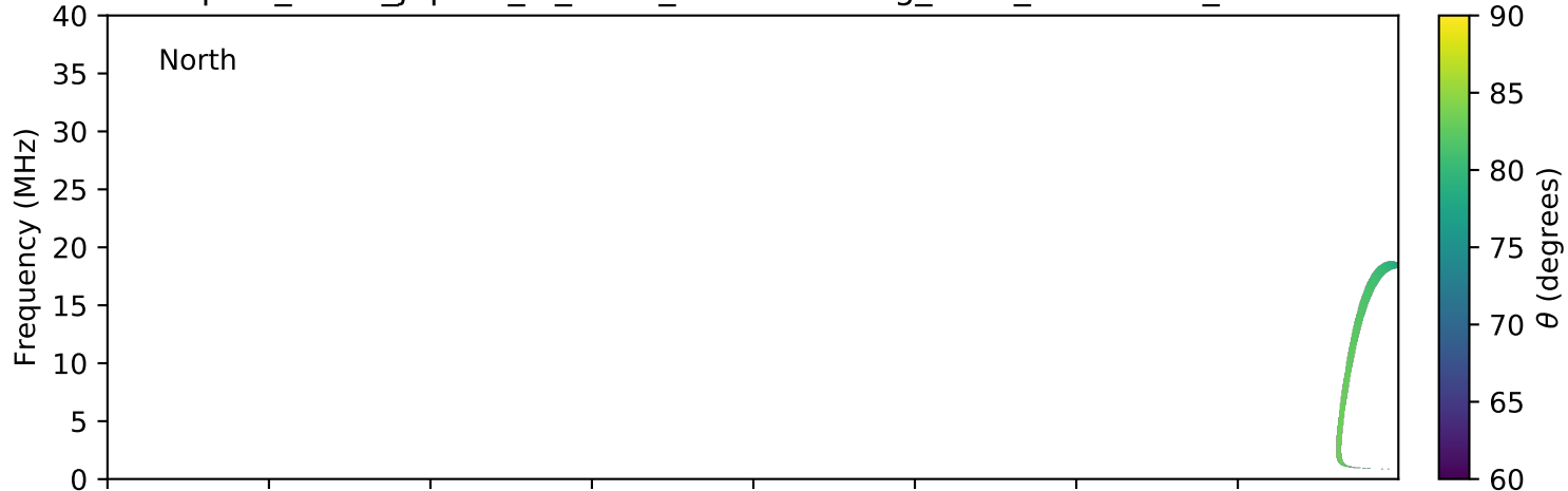
expres_earth_jupiter_io_isaac_lossc-wid1deg_3kev_20080827_v01.cdf
