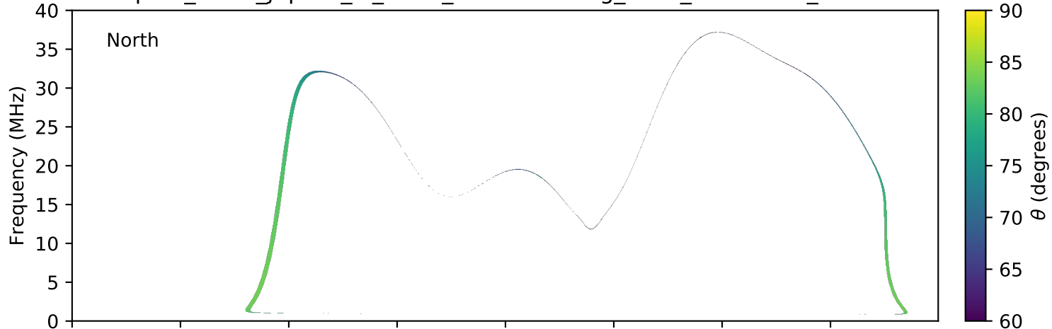
expres_earth_jupiter_io_isaac_lossc-wid1deg_3kev_20080826_v01.cdf
