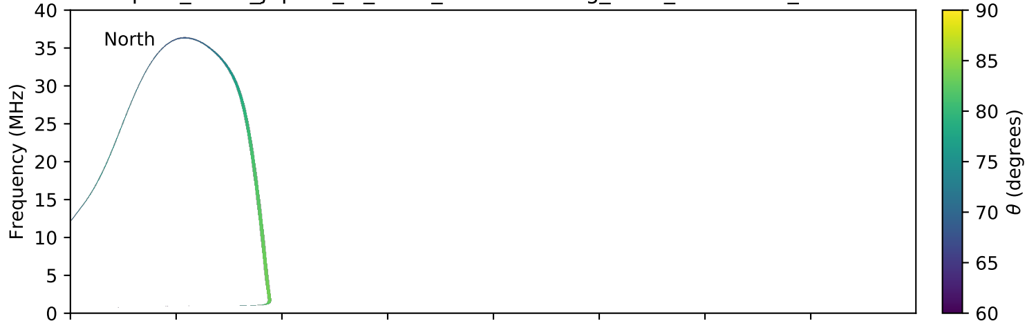
expres_earth_jupiter_io_isaac_lossc-wid1deg_3kev_20080825_v01.cdf
