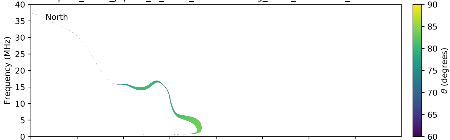
expres_earth_jupiter_io_isaac_lossc-wid1deg_3kev_20080823_v01.cdf
