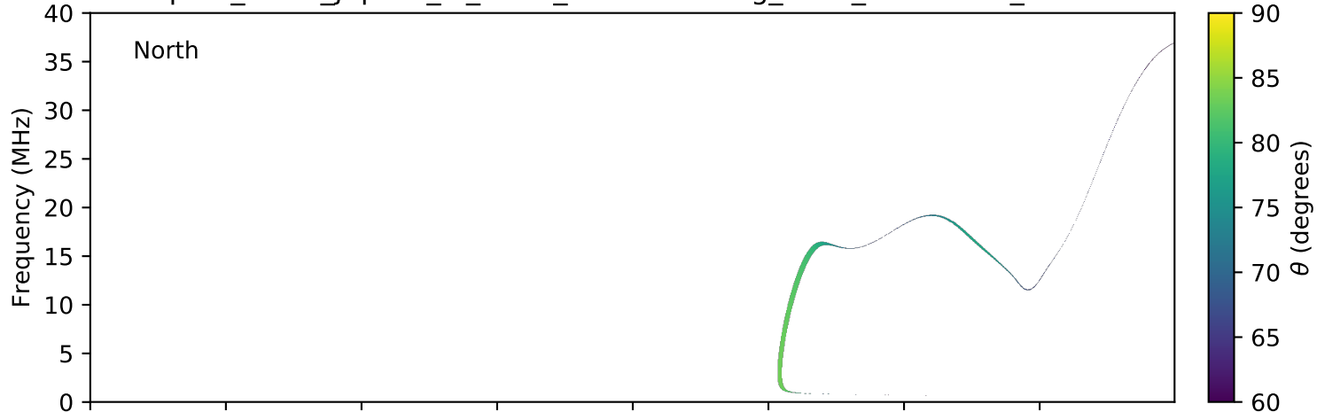
expres_earth_jupiter_io_isaac_lossc-wid1deg_3kev_20080822_v01.cdf
