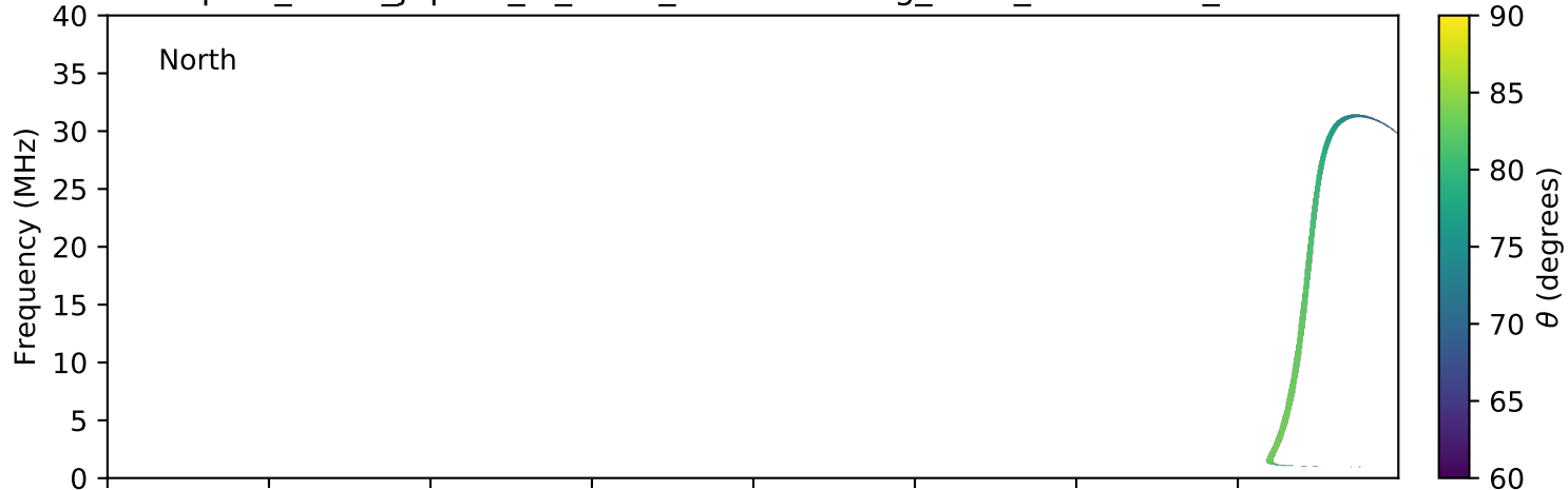
expres_earth_jupiter_io_isaac_lossc-wid1deg_3kev_20080820_v01.cdf
