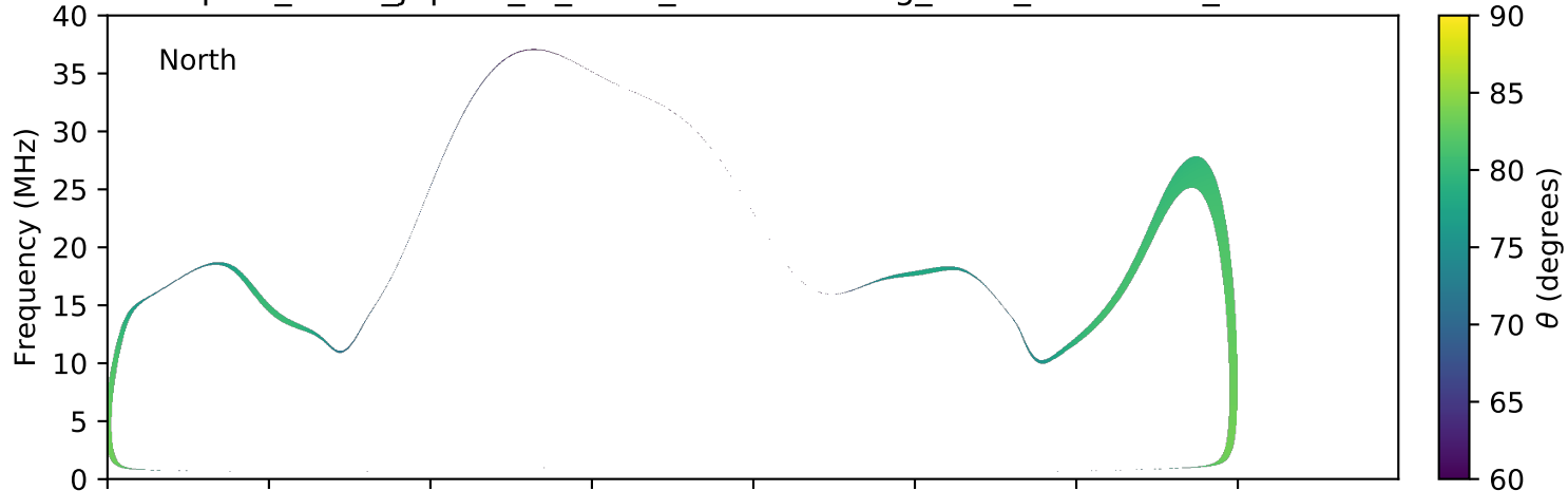
expres_earth_jupiter_io_isaac_lossc-wid1deg_3kev_20080812_v01.cdf
