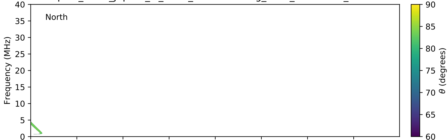
expres_earth_jupiter_io_isaac_lossc-wid1deg_3kev_20080811_v01.cdf
