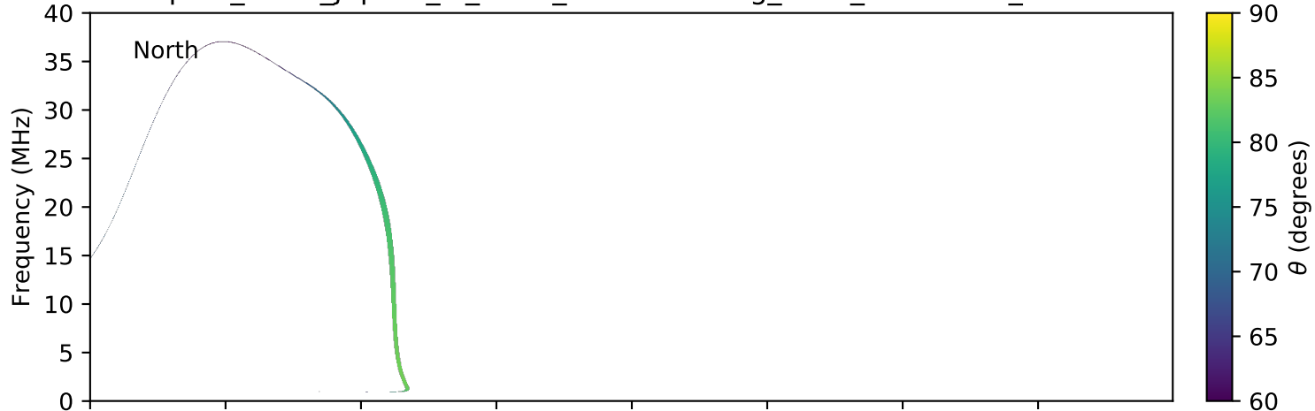
expres_earth_jupiter_io_isaac_lossc-wid1deg_3kev_20080809_v01.cdf
